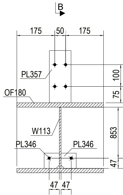
SEC A 1:10
