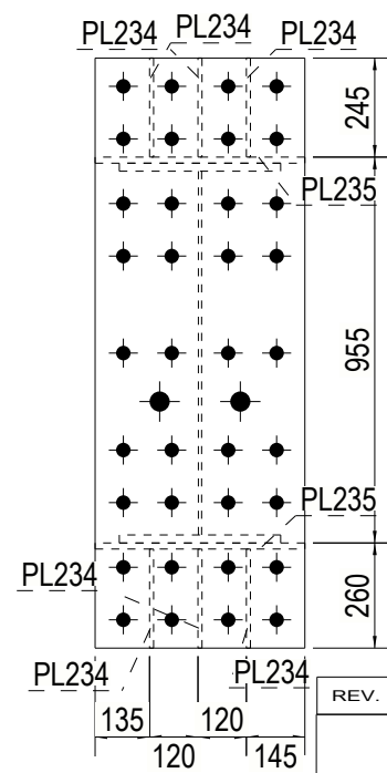
SEC C 1:20
